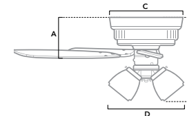
54207 | Fresh White Finish with Fresh White and Drifted Oak Blades
